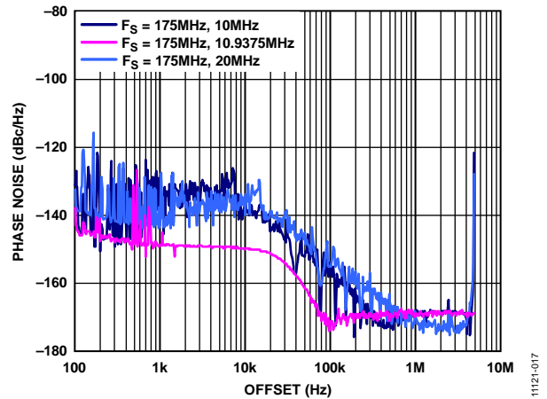
Figure 17. Phase Noise
